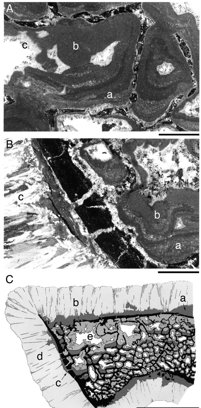
FIGURE 17. Photomicrographs and camera lucida drawing showing cross-section of Quetzalcoatlus lawsoni , sp. nov., bone (TMM 41954-1a) preserved in channel-lake facies at the Amaral Site, with typical sequence of in-filling and diagenetic features. A , photomicrographs (cross-polarized light) showing detailed filling of trabecular tissue (central part of bone shown in C ); B , adjacent to cortical tissue (lower left of bone shown in C ); C , camera lucida drawing of entire cross-section. Bone is surrounded and lower parts of vacuities are partly filled with multiple cycles of a , detrital silt and pelloidal micrite; remaining voids subsequently lined with b , clotted pustular micrite; c , late-stage cracks in cortical bone, voids; and d , exterior of bone are coated with radial-fibrous calcite; and remaining voids are filled with e , blocky equant calcite spar. Scale bars equal 1 mm ( A , B ) and 10 mm ( C ).
