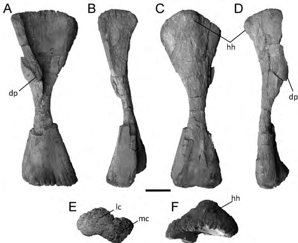
Figure 20. Nullotitan glaciensis gen. et sp. nov. Right humerus (MPM 21546) in anterior (A), lateral (B), posterior (C), medial (D), distal (E), and proximal (F) views. Abbreviations: dp, deltopectoral crest; hh, humeral head; lc, lateral condyle; mc, medial condyle. Scale bar: 10 cm.
