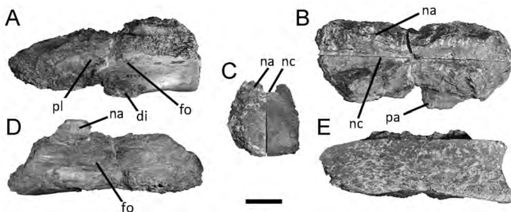
Figure 15. Nullotitan glaciaris gen. et sp. nov. Cervical vertebra (MACN Pv 18644) in left lateral (A), dorsal (B), posterior (C), right lateral (D), and longitudinal section (E) views. Abbreviations: di, diapophysis; fo, fossa; na, neural arch; nc, neural canal; pa, parapophysis; pl, pleurocoele. Scale bar: 10 cm.
