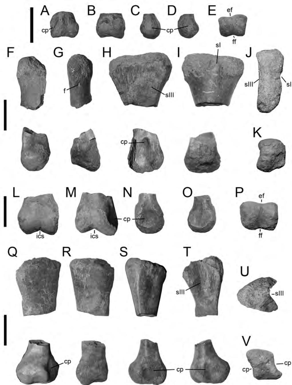
Figure 12. Isasicursor santacrucensis gen. et sp. nov. Metatarsal I in (A) anterior, (B) posterior, (C) lateral, (D) medial and (E) distal views. Proximal (above) and distal end (below) of metatarsal II (MPM 21535a) in (F) anterior, (G) posterior, (H) lateral, (I) medial (J) proximal and (K) distal views. Metatarsal III (MPM 21536) in (L) anterior, (M) posterior, (N) lateral, (O) medial and (P) distal views. Proximal (above) and distal end (below) of metatarsal IV (MPM 21537) in (Q) anterior, (R) posterior, (S) lateral, (T) medial (U) proximal and (V) distal views. Abbreviations: cp, collateral pit; ef, extensor fossa; f, foramen; ff, flexor fossa; ics, intercondylar sulcus; sl, surface for the mtt I; sIII, surface for the mtt III. Scale bar: 3 cm.
