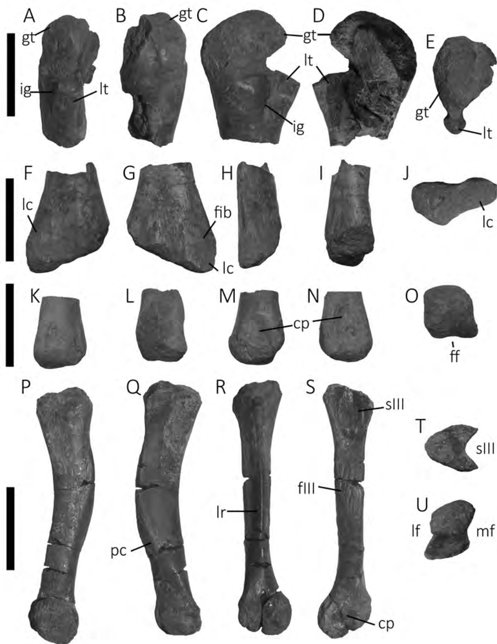
Figure 11. Isasicursor santacruzensis gen. et sp. nov. Selected juvenile materials. Right femur (MPM 21533b) in (A) anterior, (B) posterior, (C) lateral (D) medial and (E) proximal views. Left tibia (MPM 21534b) in (F) anterior, (G) posterior, (H) lateral (I) medial and (J) distal views. Metatarsal II in (K) anterior, (L) posterior, (M) lateral (N) medial and (O) distal views. Metatarsal IV (MPM 21538b) in (P) anterior, (Q) posterior, (R) lateral (S) medial (T) proximal and (U) distal views. Abbreviations: cp, collateral pit; fib, fibular facet; gt, greater trochanter; ig, intertrochanteric groove; lc, lateral condyle; lf, lateral fossa; lr, lateral ridge; lt, lesser trochanter; mf, medial fossa; pc, plantar crest; sIII, surface for mtt III. Scale bar: 3 cm.
