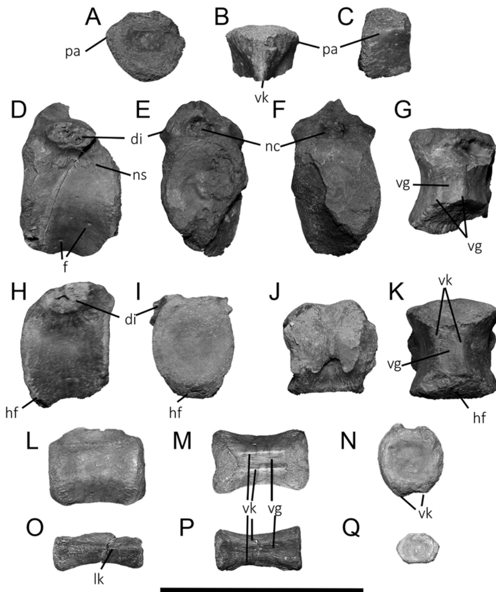
Figure 8. Isasicursor santacruzensis gen. et sp. nov. Selected vertebral elements. Cervical vertebra (MPM 21526) in (A) anterior, (B) ventral and (C) lateral. Dorsal Vertebra (MPM 21527) in (D) lateral, (E) anterior, (F) posterior and (G) ventral views. Proximal caudal vertebra (MPM 21529) in (H) lateral, (I) anterior, (J) dorsal and (K) ventral views. Middle caudal vertebra (MPM 21529) in (L) lateral, (M) ventral and (N) anterior views. Posterior caudal vertebra (MPM 21529) in (O) lateral, (P) ventral and (Q) anterior views. Abbreviations: di, diapophysis; hf, haemal facet; lk, lateral keel; nc, neural canal; ns, neural suture; vg, ventral groove; vk, ventral keel. Scale bar: 5 cm.
