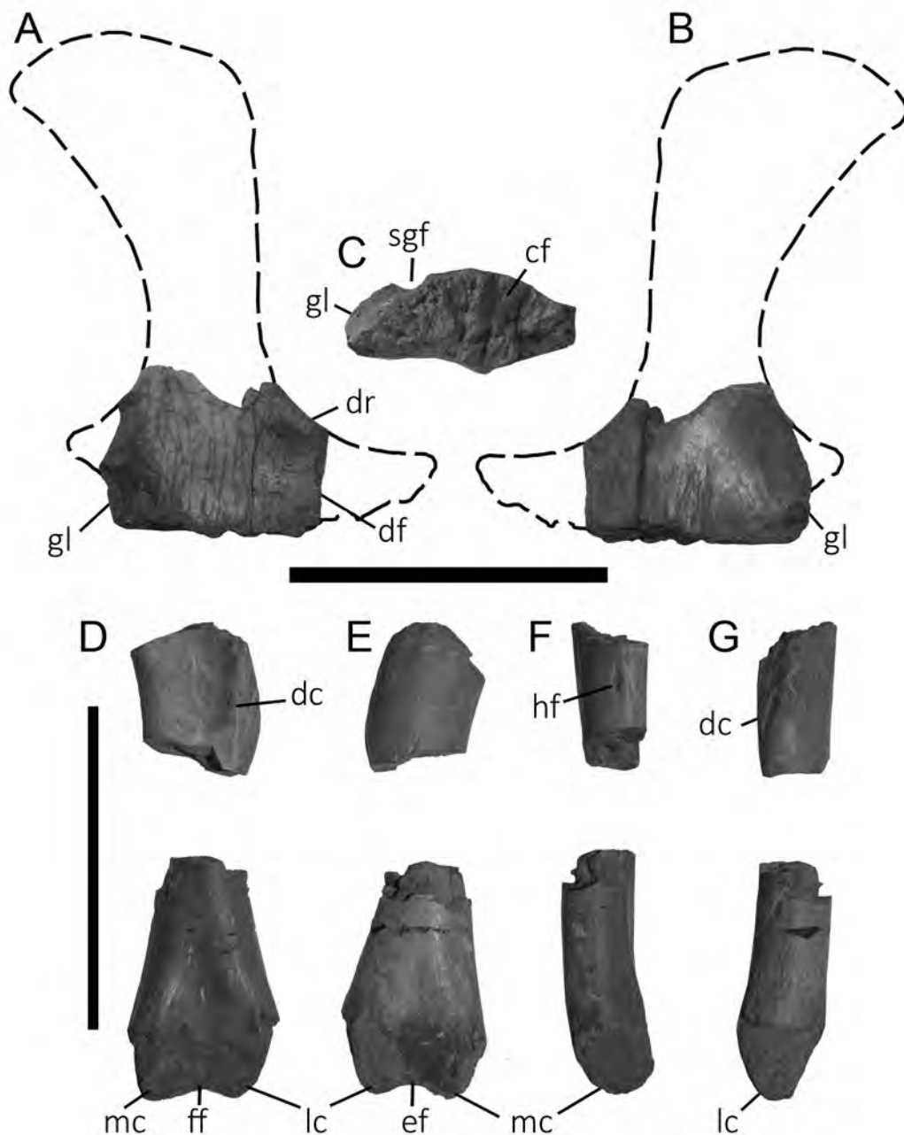
Figure 10. Isasicursor santacrucensis gen. et sp. nov. Scapula (MPM 21530) in (A) lateral (B), medial and (C) coracoid views. Humerus (MPM 21531) in (D) anterior, (E) posterior, (F) medial and (G) lateral views. Abbreviations: dc, deltopectoral crest; df, deltoid fossa; dr, deltoid rim; ef, extensor fossa; ff, flexor fossa; gl, glenoid fossa; hf, humeral foramen; lc, lateral condyle; mc, medial condyle; sgf, supraglenoid fossa. Scale bar: 10 cm.
