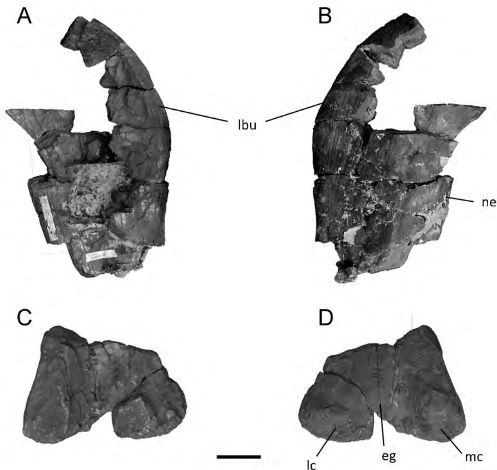
Figure 21. Nullotitan glaciensis gen. et sp. nov. Proximal (A-B) and distal (C-D) ends of right femur (MPM 21542) in anterior (A, C), and posterior (B, D) views. Abbreviations: eg, extensor groove; lc, lateral condyle; lbu, lateral bump; mc, medial condyle; ne, neck. Scale bar: 10 cm.
