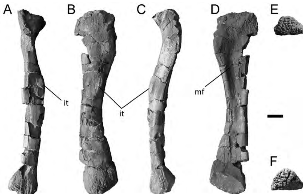
Figure 23. Nullotitan glaciaris gen. et sp. nov. Right fibula (MPM 21542) in anterior (A), lateral (B), posterior (C), medial (D), proximal (E), and distal (F) views. Abbreviations: it, iliofibularistubercle; mf, medial fossa. Scale bar 10 cm.
