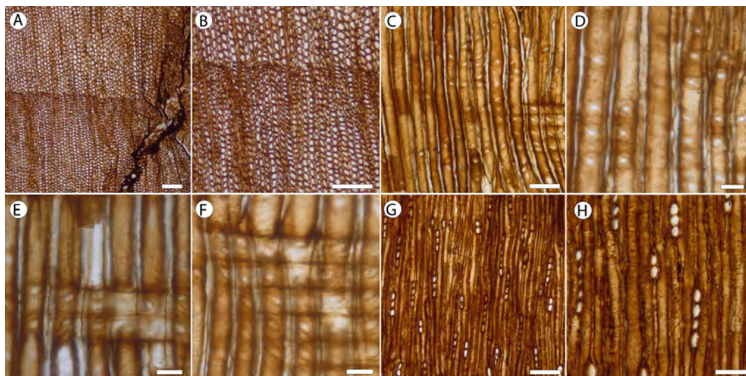
Figure 33. Podocarpoxylon dusenii Krausel 1924. A , (MPM 21568) Growth ring in a transverse section (TS). Bar: 20 \mu m. B , (MPM 21568) Detail of growth ring (TS). Bar: 20 \mu m. C , (MPM 21567) Spaced uniseriate radial pitting and cross fields (LRS). Bar: 50 \mu m. D , (MPM 21567) Spaced uniseriate radial pitting and cross fields (LRS). Bar: 20 \mu m. E , F , (MPM 21567) Cross fields with 1 or 2 podocarpoid pits (LRS). Bar: 20 \mu m. G , (MPM 21567) Uniseriate rays (LTS). Bar: 20 \mu m. H , (MPM 21567) Detail of uniseriate rays (LTS). Scale bar: 50 \mu m
