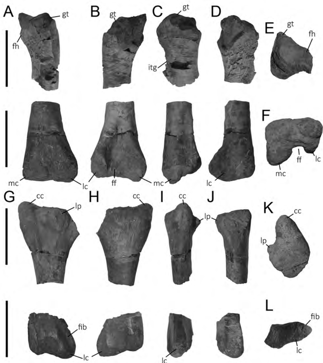
Figure 7. Isasicursor santacrucensis gen. et sp. nov. Femur (MPM 21533a) in (A) anterior, (B) posterior, (C) lateral, (D) medial, (E) proximal and (F) distal views. Tibia (MPM 21525a) in (G) lateral, (H) medial, (I) anterior, (J) posterior, (K) proximal and (L) distal views. Abbreviations: cc, cnemial crest; fib, fibular facet; ff, flexor fossa; fh, femoral head; gt, greater trochanter; itg, intertrochanteric groove; lc, lateral condyle; lp, lateral process; mc, medial condyle. Scale bar: 10 cm.
